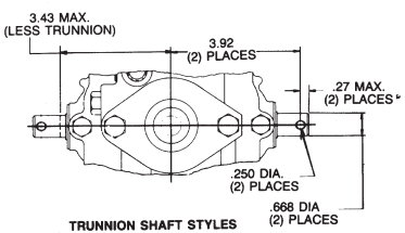
TRUNNION SHAFT STYLES
