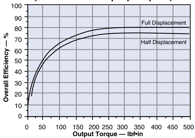
15 "U" Overall Efficiency (@ 3300 RPM Pump Input Speed)
